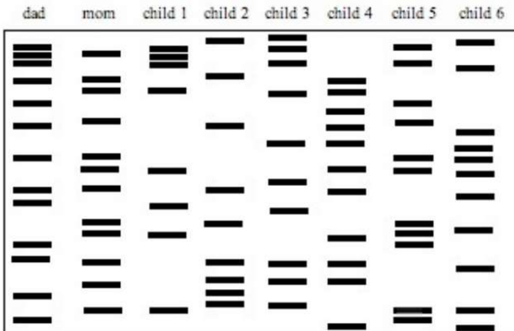
DNA Fingerprint #5
