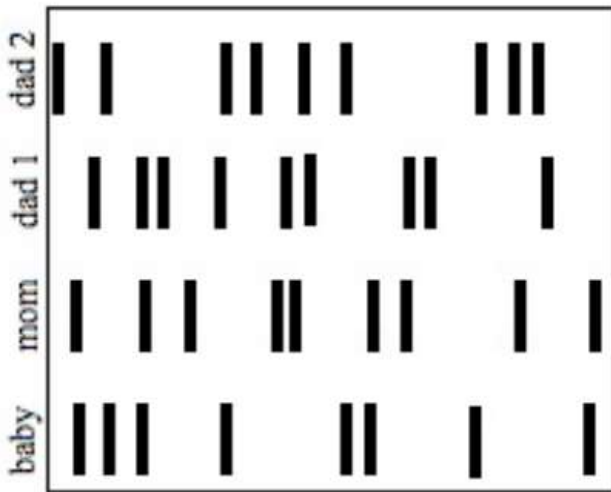
DNA Fingerprint #3
