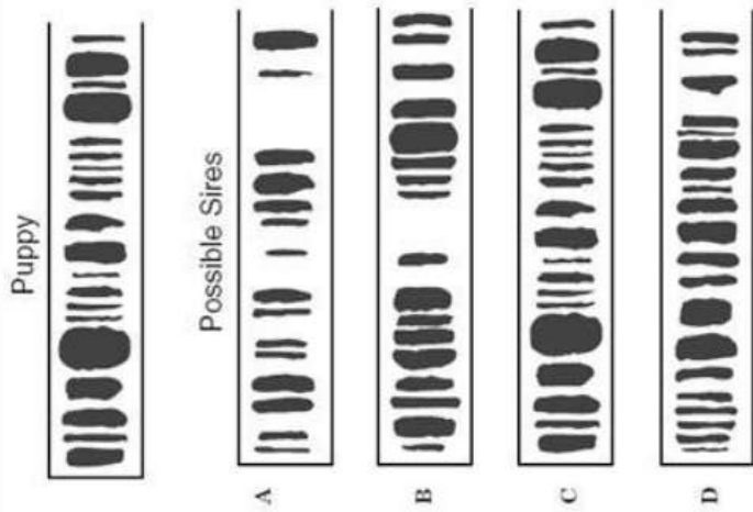
DNA Fingerprint #1
