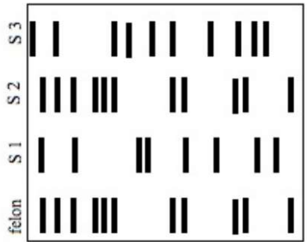
DNA Fingerprint #2
