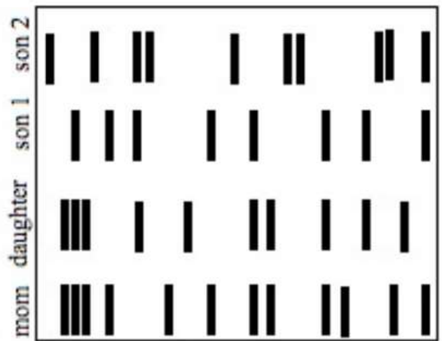
DNA Fingerprint #4
